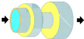
Figure 3: Three-dimensional cross-section for Four-segments muffler
