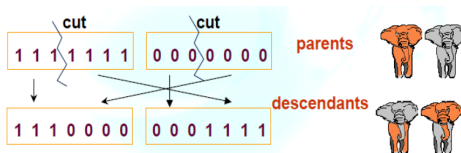
Figure 12: Single point Crossover
