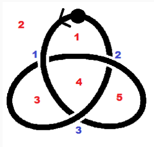
Figure 2: Labeled Trefoil
