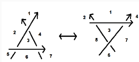
Figure 6: Reidemeister 3 move
